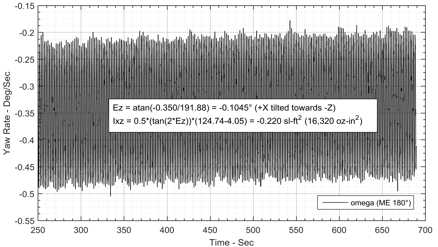
Figure 3-16. Yaw Rate vs Time
