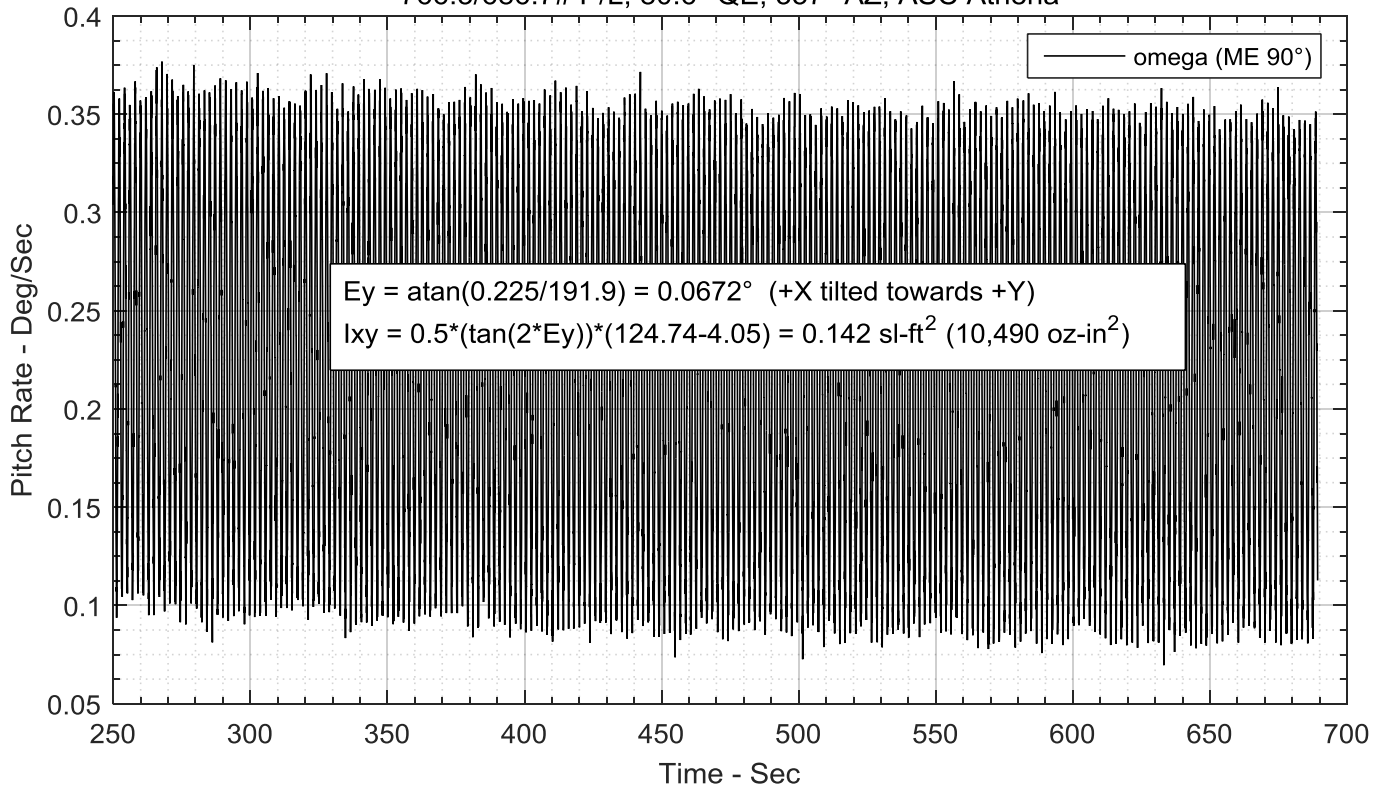
Figure 3-15. Pitch Rate vs Time
